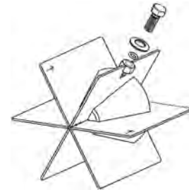
Figure 9. Flow Straightener
