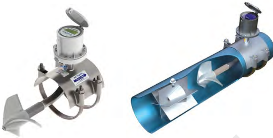
McCrometer brand McPropeller Flow Meter (left) and FS100 flow straightening vane (right)
