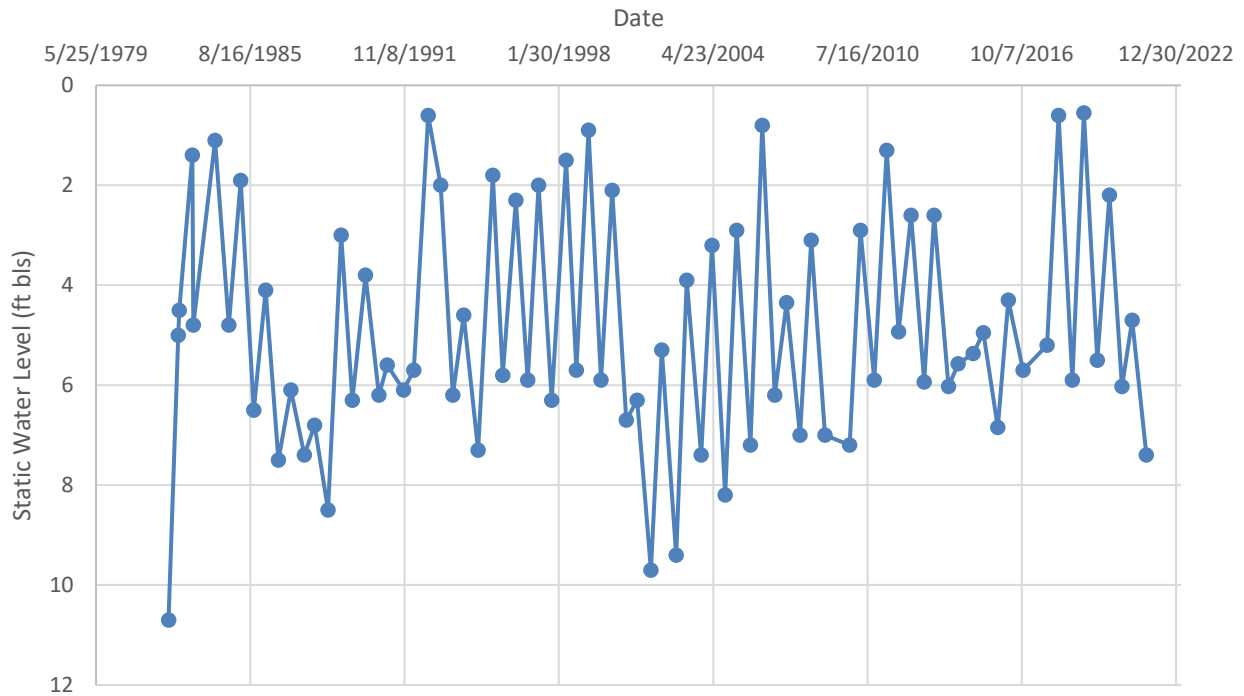
Existing Well Historic Static Water Levels (1980-2021)
