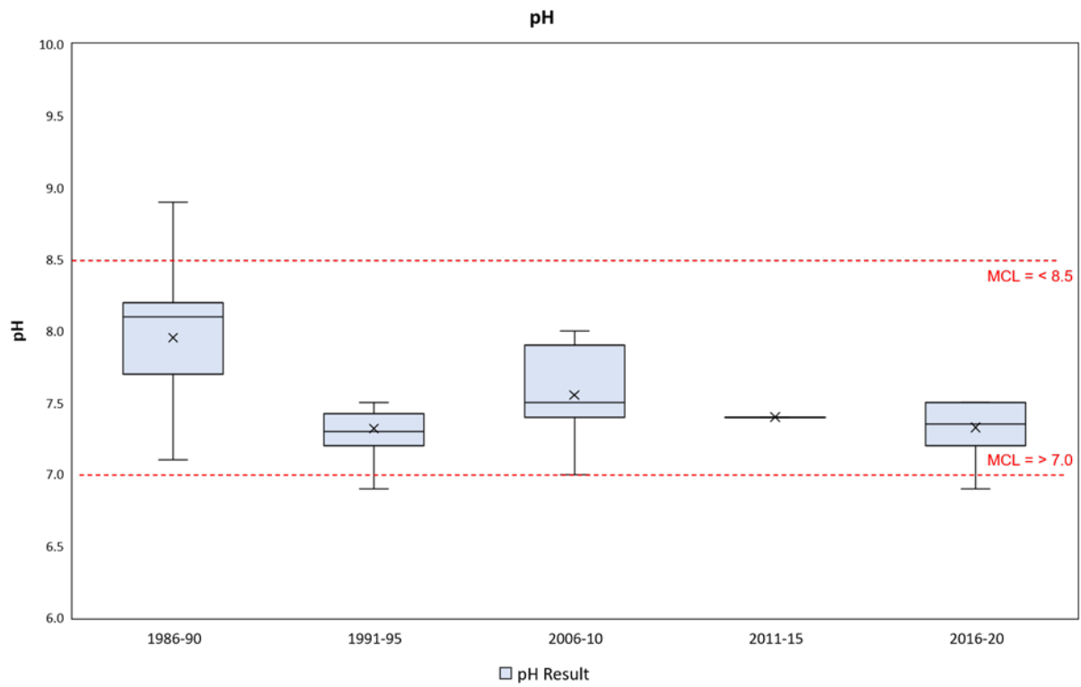
Figure A##-5. pH, Groundwater Quality Observations (1990 – 2020)
