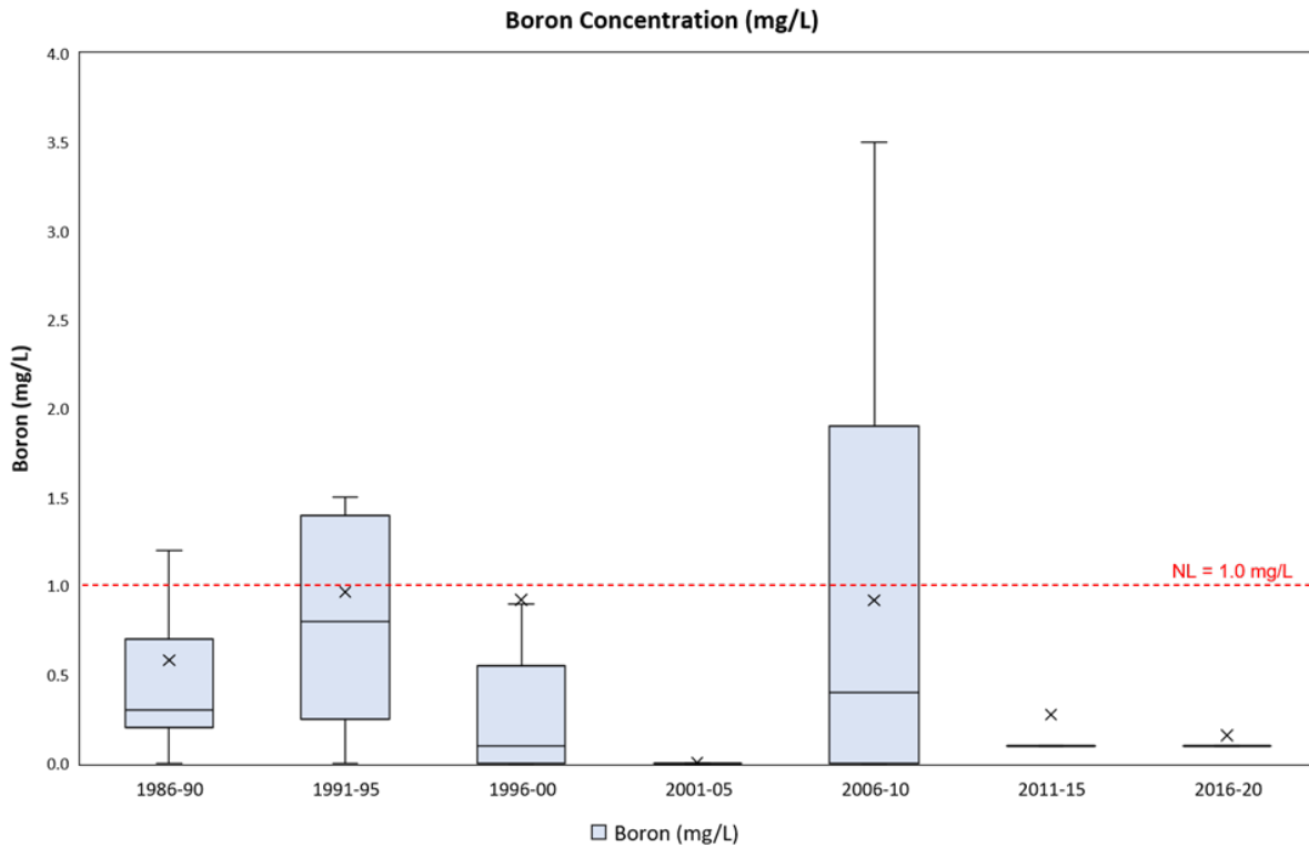
Figure A##-4. Boron, Groundwater Quality Observations (1990 – 2020)
