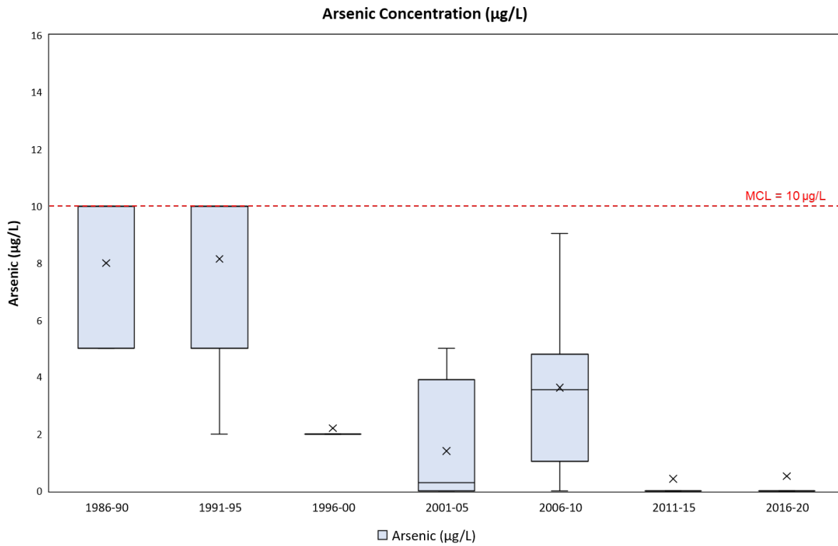
Figure A##-3. Arsenic, Groundwater Quality Observations (1990 – 2020)
