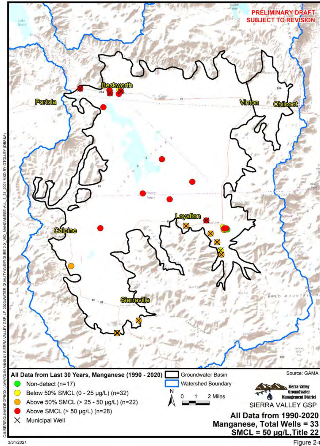
Figure A##-21. Manganese, Maximum Groundwater Quality Observations (1990 – 2020)
