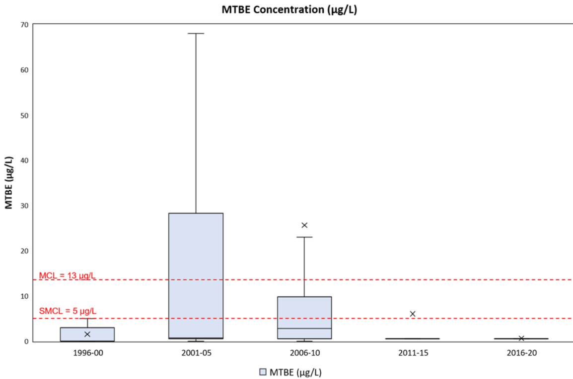
Figure A##-8. MTBE, Groundwater Quality Observations (1990 – 2020)
