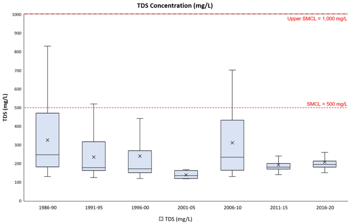
Figure A##-2. TDS, Groundwater Quality Observations (1990 – 2020)
