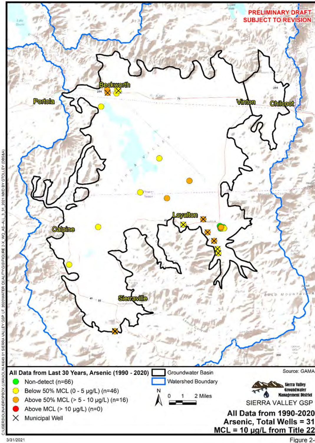
Figure A##-13. Arsenic, Maximum Groundwater Quality Observations (1990 – 2020)
