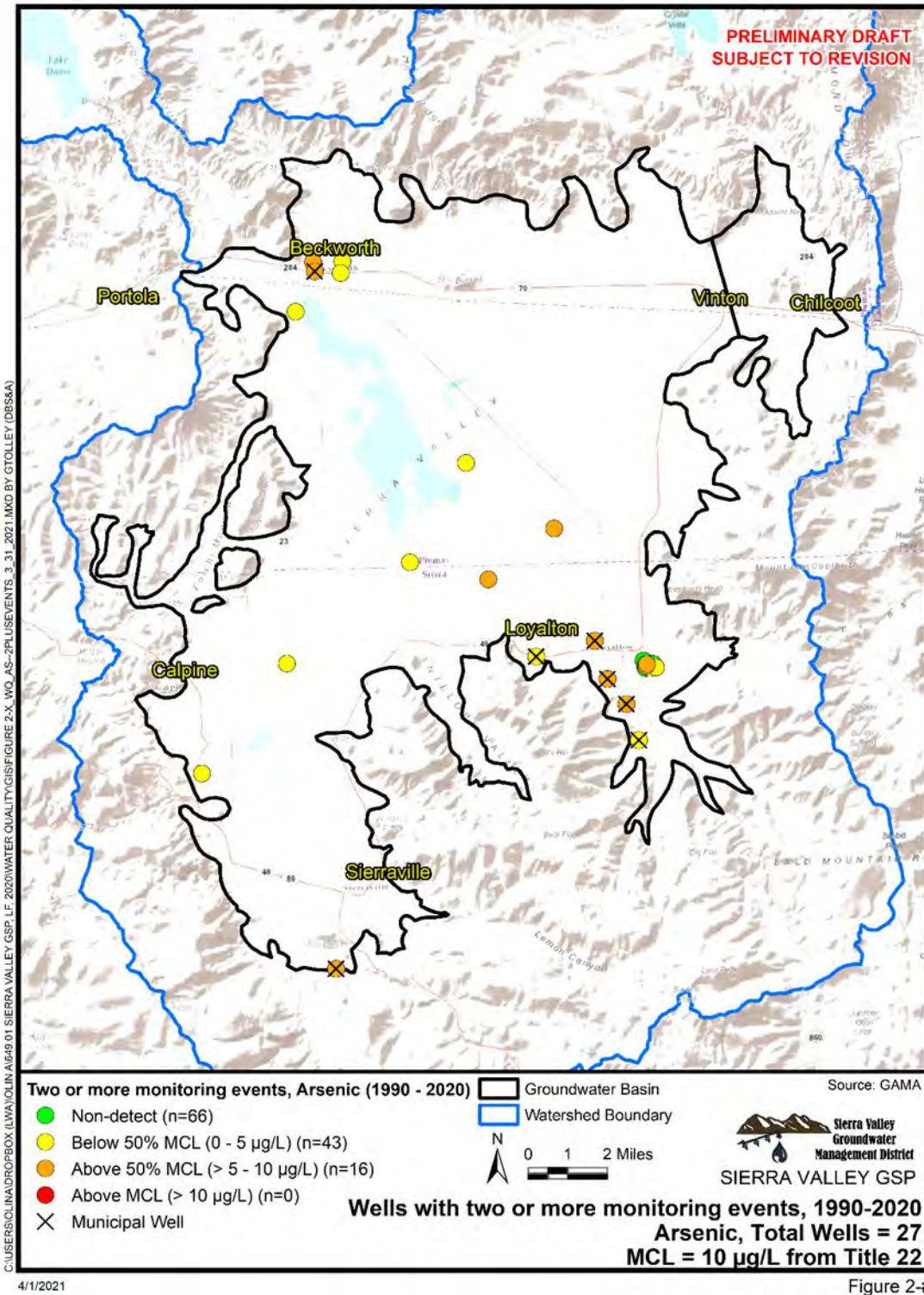
Figure A##-14. Arsenic, Maximum Groundwater Quality Observations from Wells with Two or More Measurements (1990 – 2020)
