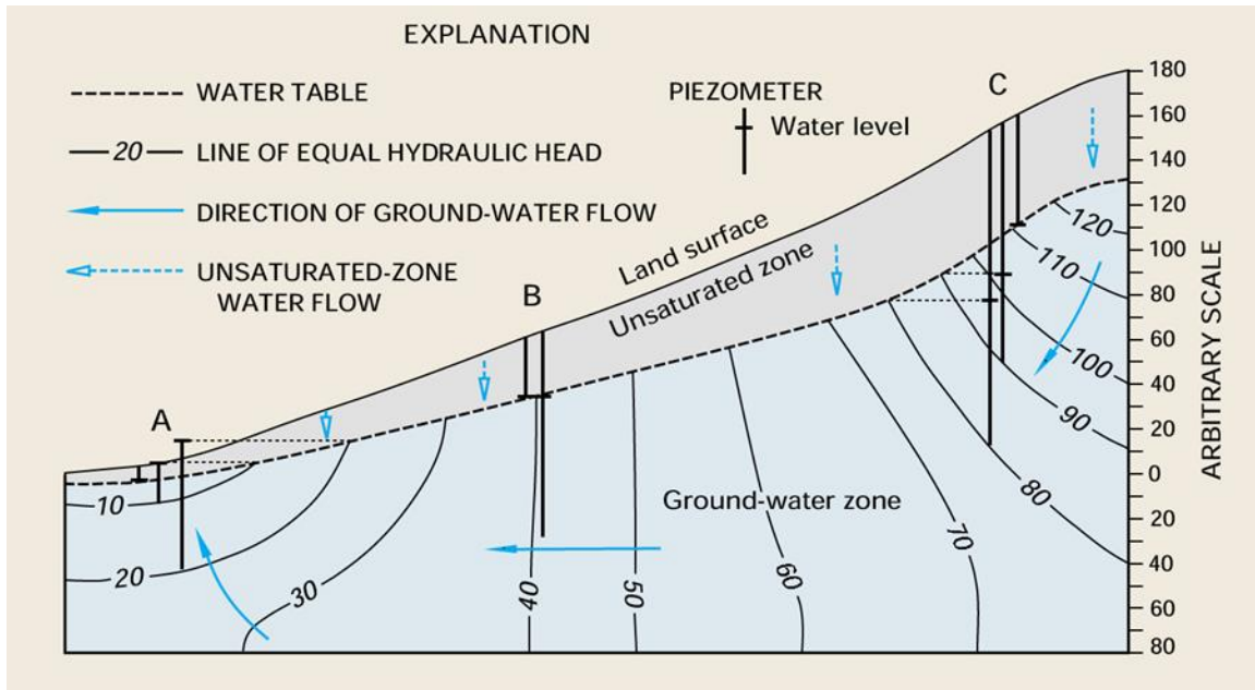
Figure 4-1 - Conceptual depiction of a typical groundwater flow system. From Winter et al. (1998).
