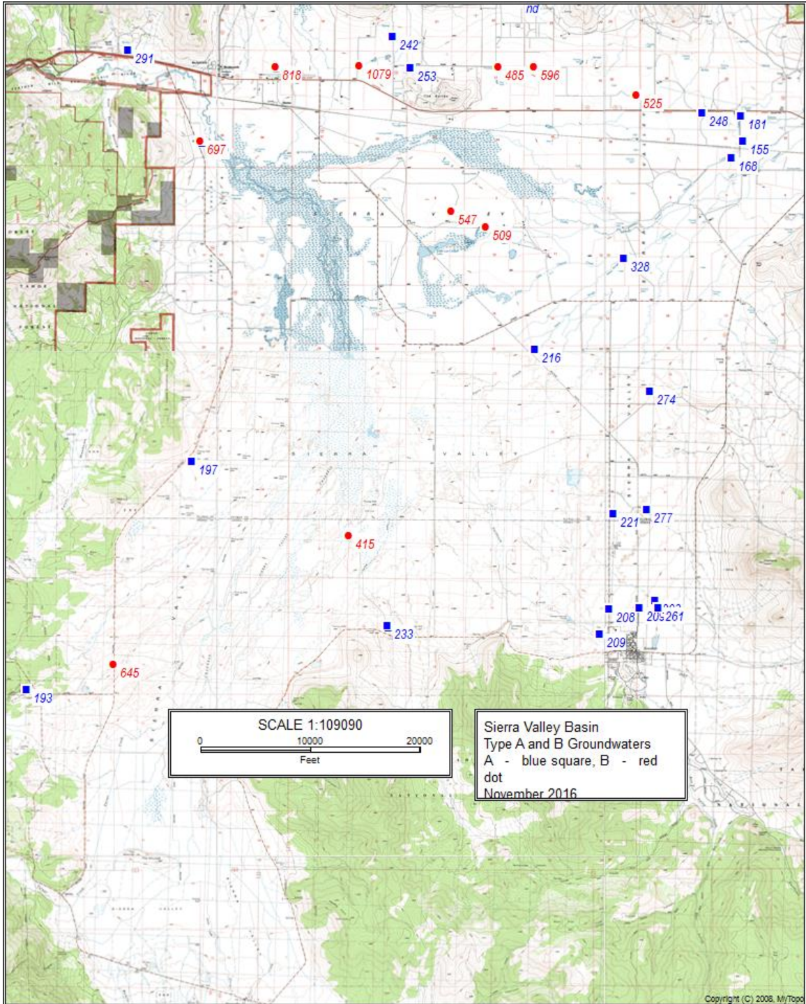
Map 4-2 Type A and Type B groundwaters, Sierra Valley. the labels are field electric conductivity at time of sampling. For explanations see text.
