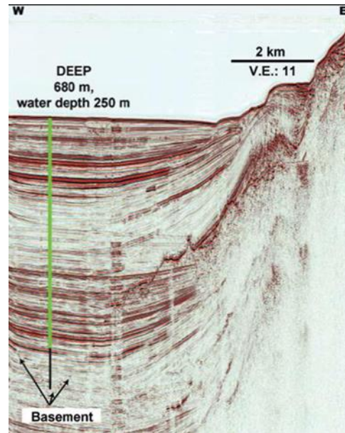
Figure 3-3 Seismic profile of Lake Ohrid sediments deposited while the underlying bedrock basement is subsiding. From Wagner et al. (2014).
