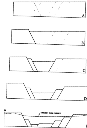
Figure 3-1 The development of a fault trough (from Thompson et al., 1967).
