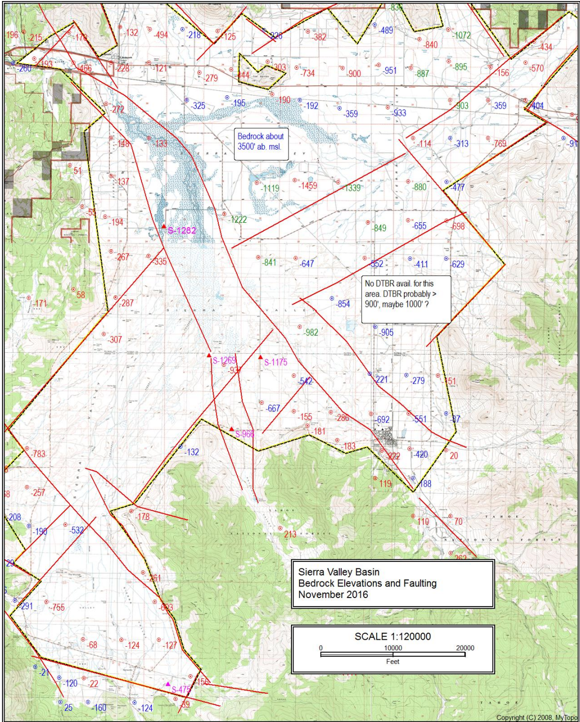
Map 3-1 Sierra Valley Basin bedrock topography and faults. Red labels are average bedrock elevation in feet above the 5000 ft elevation datum for each one-square mile section indicated by a red dot (negative numbers indicate bedrock elevation is less than 5000 ft). Blue and green labels indicate approximate maximum bedrock elevations.
